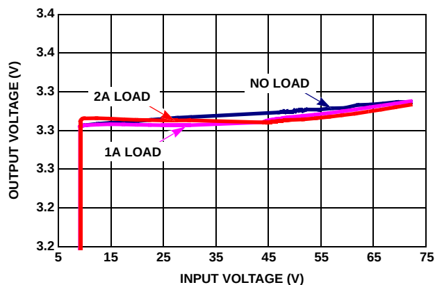
FIGURE 16. OUTPUT VOLTAGE REGULATION vs V_{IN} (PWM MODE)
