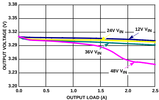
FIGURE 8. V_{OUT} REGULATION vs LOAD ( V_{OUT} = 3.3V - 500kHz)
