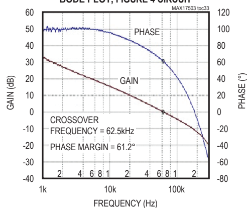
5V OUTPUT, 2.5A LOAD CURRENT BODE PLOT, FIGURE 4 CIRCUIT
