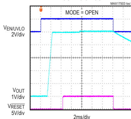
3.3V OUTPUT, PFM MODE SOFT-START WITH 2.5V PREBIAS, FIGURE 4 CIRCUIT
