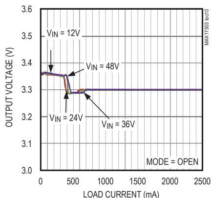
3.3V OUTPUT, PFM MODE, FIGURE 4 CIRCUIT LOAD AND LINE REGULATION
