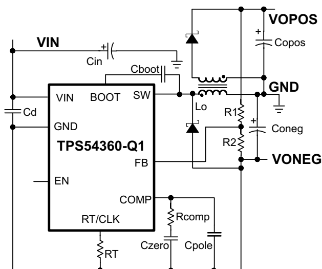
Figure 56. TPS54360-Q1 Split Rail Power Supply based on Application Note (SLVA369)
