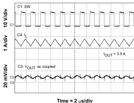
Figure 39. Output Ripple CCM
