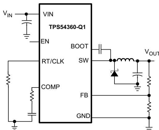
SIMPLIFIED SCHEMATIC
