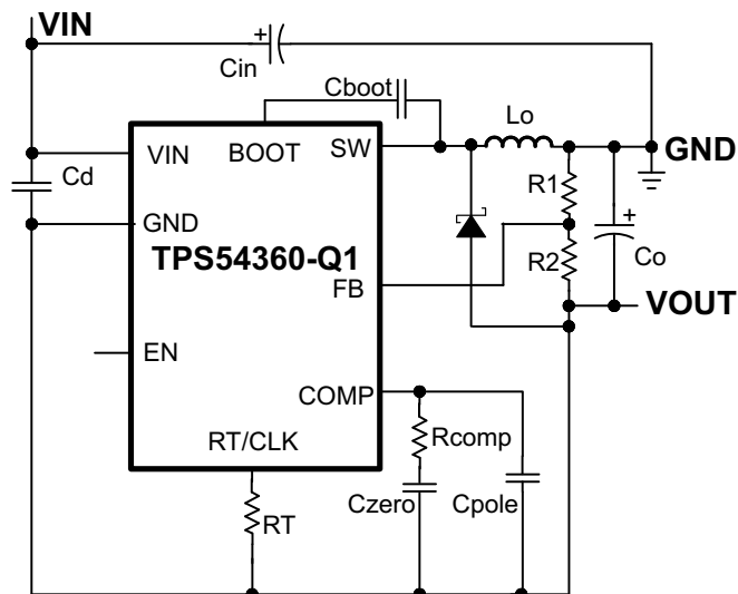
Figure 55. TPS54360-Q1 Inverting Power Supply based on Application Note (SLVA317)
