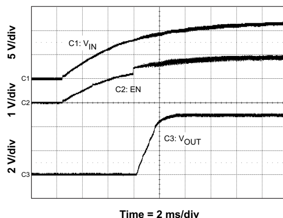
Figure 37. Startup With VIN
