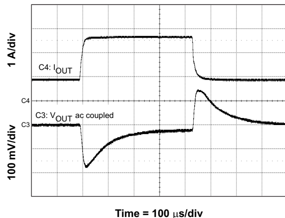
Figure 35. Load Transient
