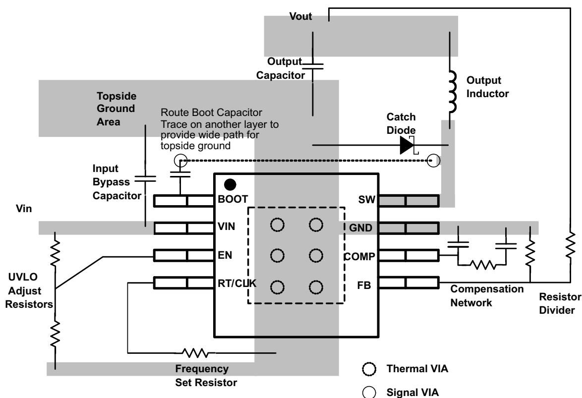
Figure 54. PCB Layout Example
