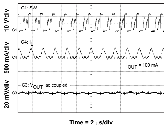
Figure 40. Output Ripple DCM
