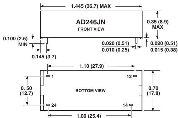
CONTROLLING DIMENSIONS ARE IN INCHES; MILLIMETER DIMENSIONS (IN PARENTHESES) ARE ROUNDED-OFF MILLIMETER EQUIVALENTS FOR REFERENCE ONLY AND ARE NOT APPROPRIATE FOR USE IN DESIGN
