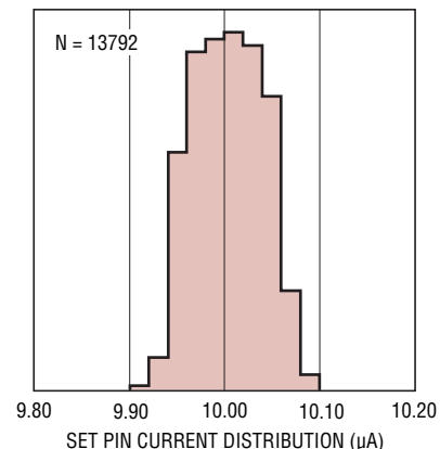
Set Pin Current Distribution
