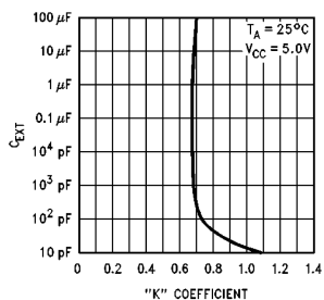
DM74LS221
