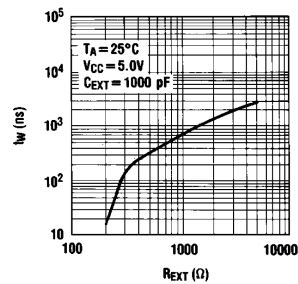
DM74121
