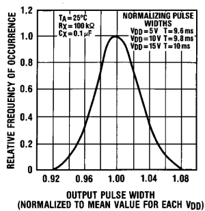
Typical Normalized Distribution of Units for Output Pulse Width
