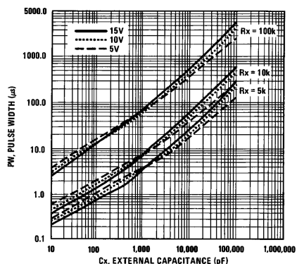
Pulse Width vs. C_X
