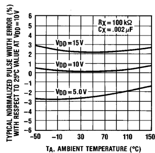
Typical Pulse Width Error vs. Temperature
