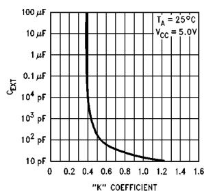
DM74LS123
