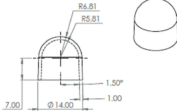
Mechanical Diagram, DOM60
