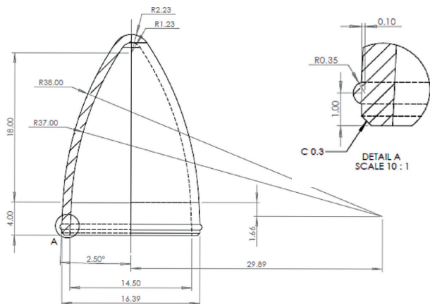
Mechanical Diagram, CAN30
