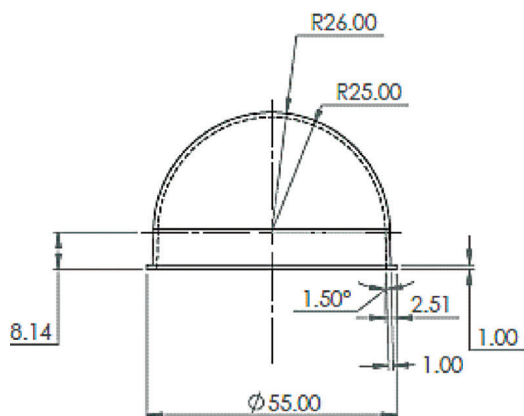
Mechanical Diagram, DOM60
