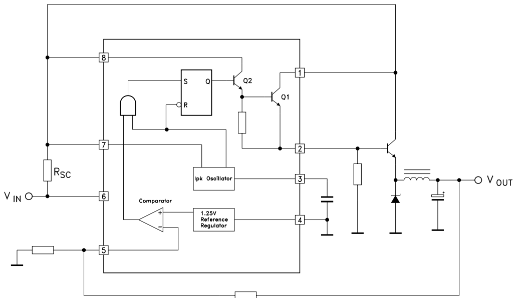
Figure 20. Step-down with external NPN switch
