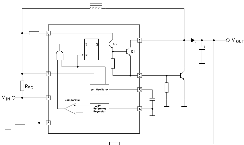
Figure 19. Step-up with external NPN switch
