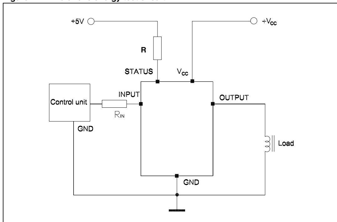
Figure 7. Avalanche energy test circuit
