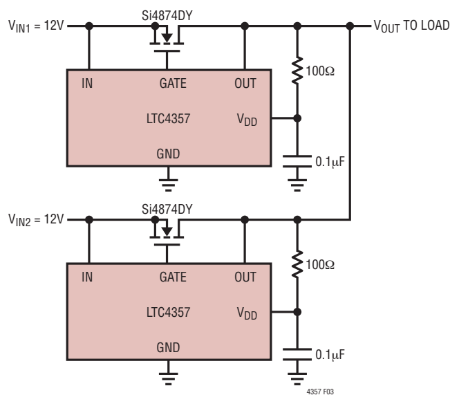
Figure 3. 12V, 10A Diode-OR
