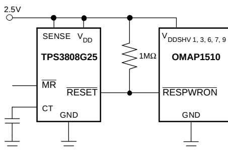
Figure 11. Typical Application of the TPS3808 with an OMAP Processor
