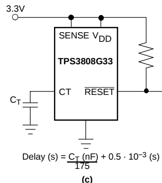
Figure 15. Configuration Used to Set the \overline{\text{RESET}} Delay Time
