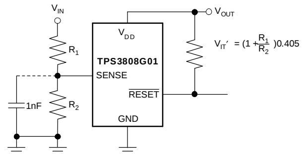
Figure 12. Using the TPS3808G01 to Monitor a User-Defined Threshold Voltage
