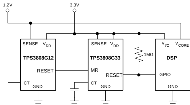
Figure 13. Using \overline{\text{MR}} to Monitor Multiple System Voltages
