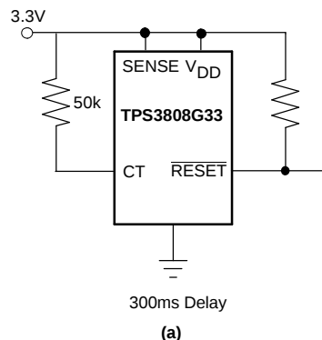
Figure 15. Configuration Used to Set the \overline{\text{RESET}} Delay Time
