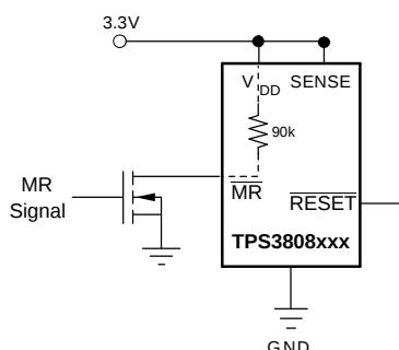
Figure 14. Using an External MOSFET to Minimize \text{I}_{\text{DD}} When \overline{\text{MR}} Signal Does Not Go to \text{V}_{\text{DD}}
