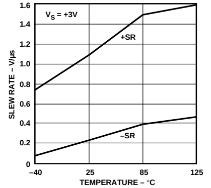
Figure 16. Slew Rate vs. Temperature, V_S = +3\text{ V}
