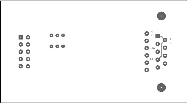
Figure 7d. Low EMI Demo Board Layout (DC1747A), Inner Layer 2
