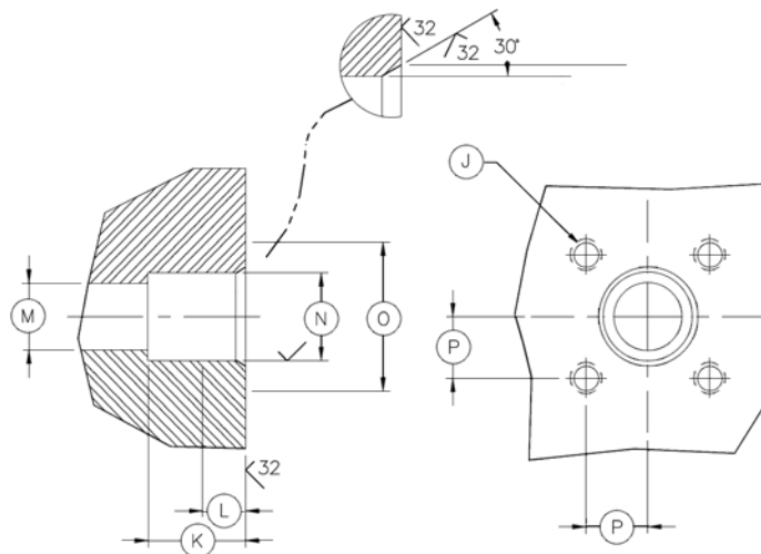
FCR INTERFACE MOUNTING INFORMATION
