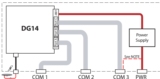
Fig. 1.5. DG14 Sensor Power-I/O Connections
