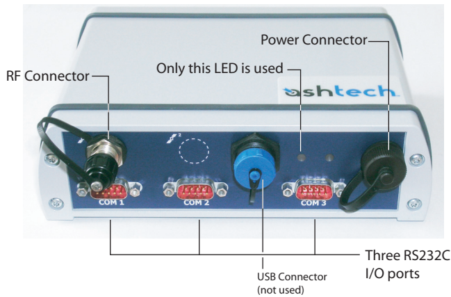
Fig. 1.2. ProFlex Lite-DG14 Sensor
