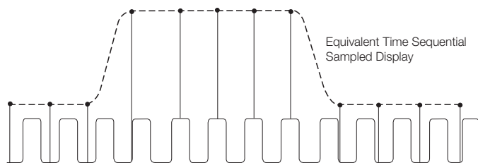
Figure 32. In sequential equivalent-time sampling, the single sample is taken for each recognized trigger after a time delay which is incremented after each cycle.
