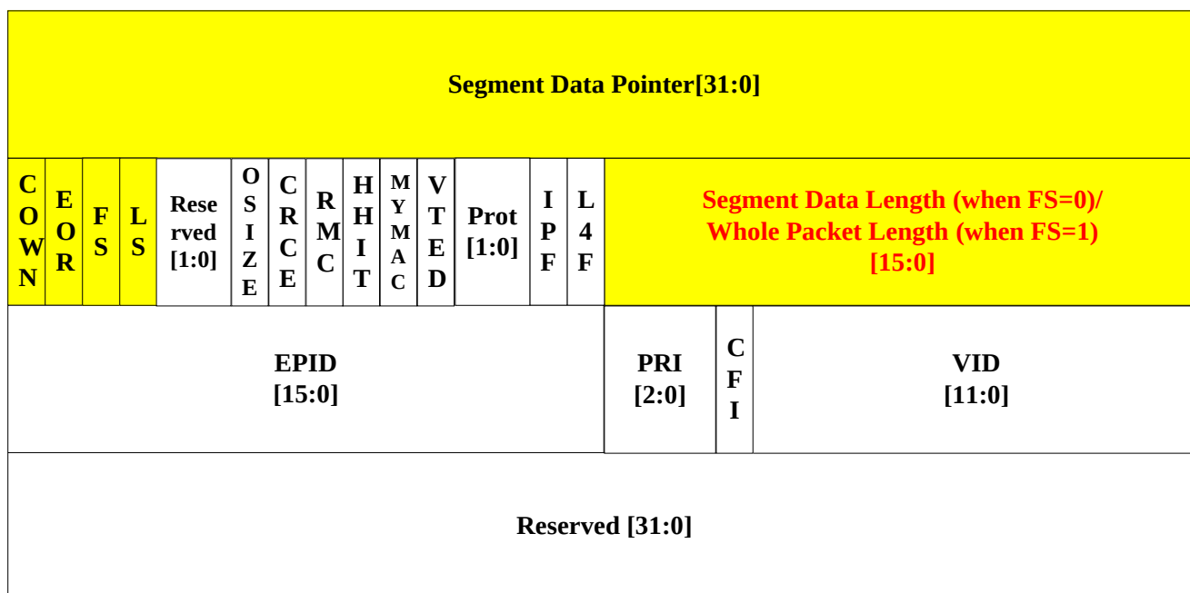
Figure 9. RX Descriptor Format
