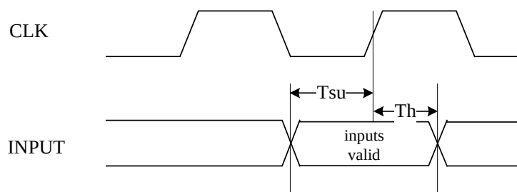
Figure 35. PCI Interface Timing
