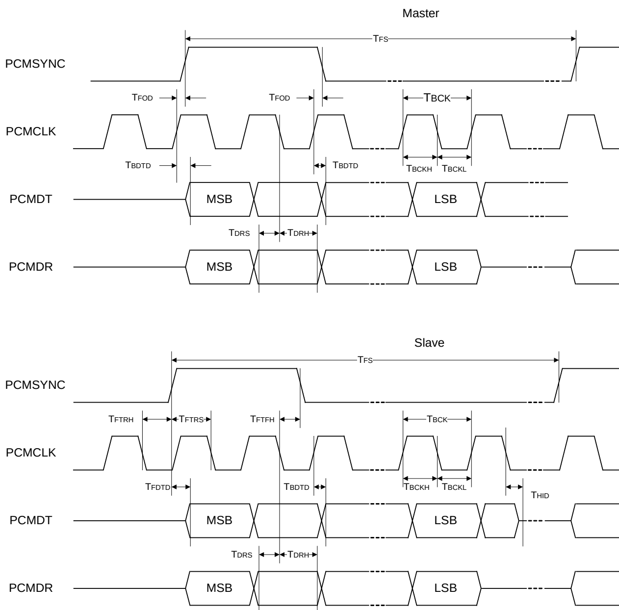
Figure 41. Long Frame Sync PCM
