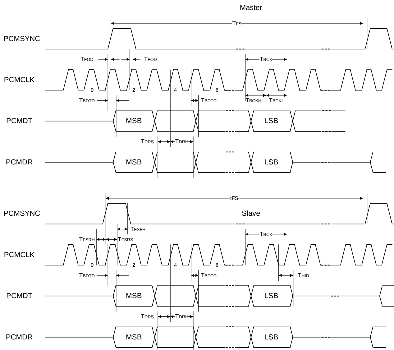
Figure 43. GCI PCM
