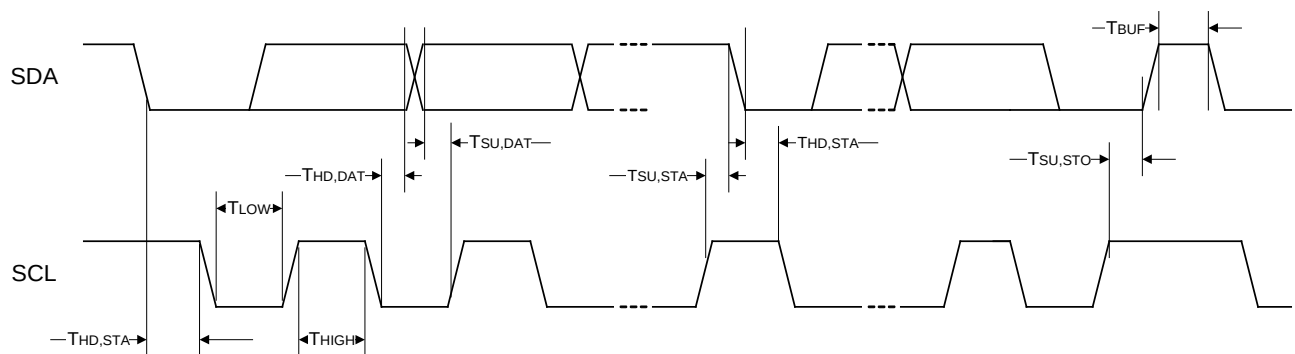
Figure 36. TWI Read
