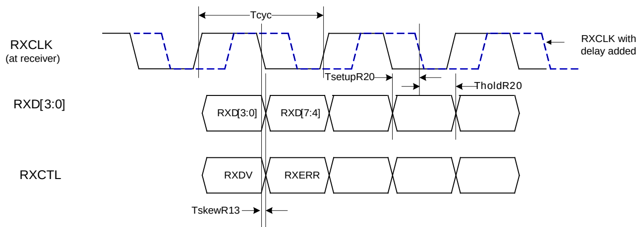
Figure 45. RGMII Interface Timing Diagram
