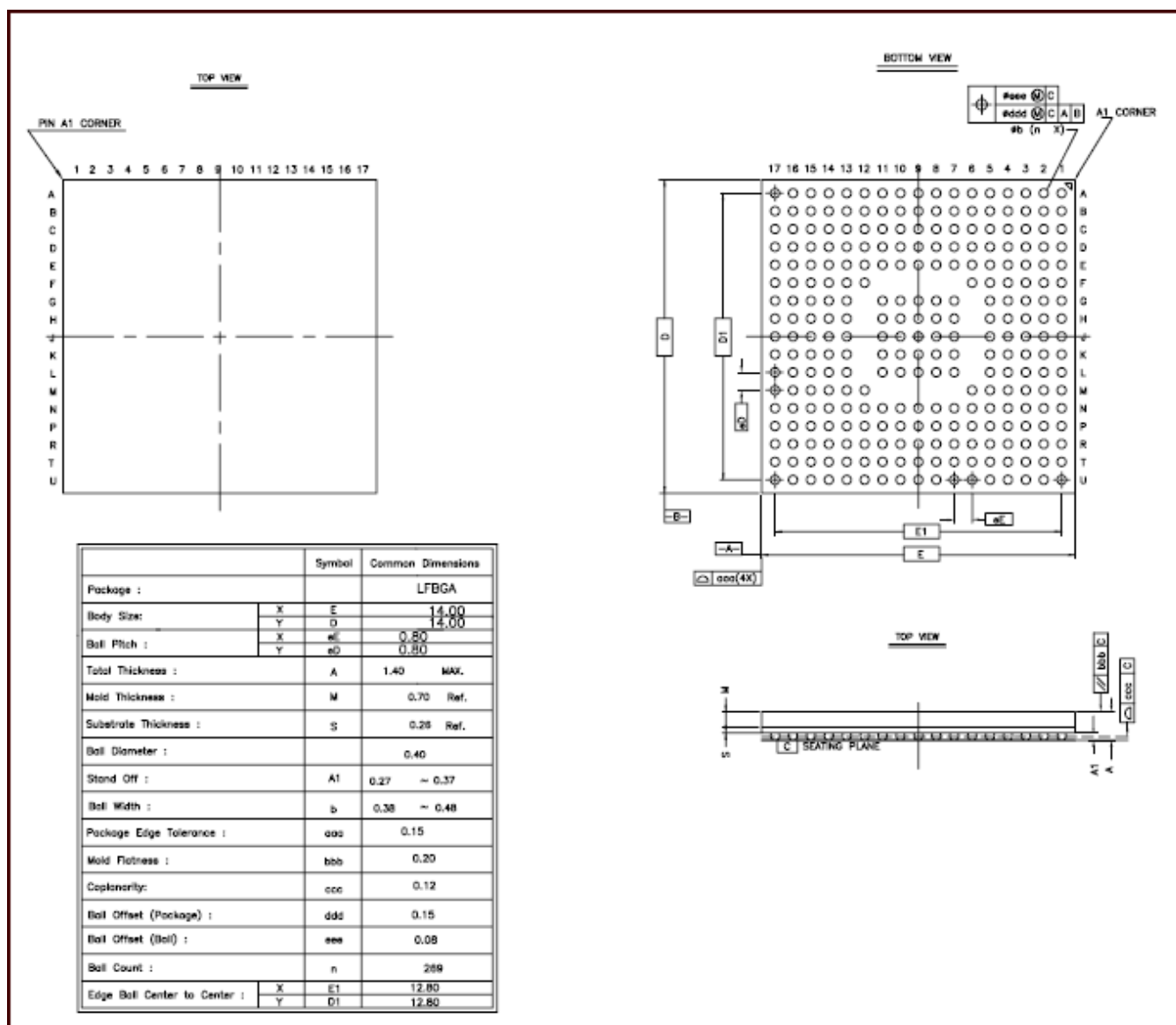
Figure 51. STR8182/CNS2182, STR8182X/CNS2182X Package Outline and Dimensions-LFBGA-269
