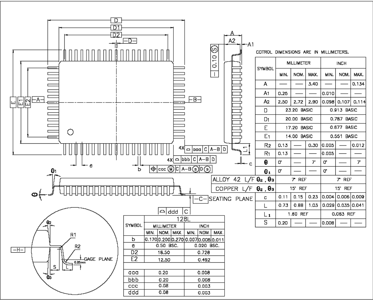
Figure 50. STR8131/CNS2131, STR8132/CNS2132, STR8181/CNS2181 Package Outline and Dimensions—PQFP-128
