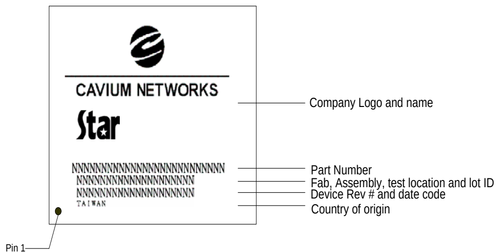
Figure 57. STR81XX /CNS21XX Package Marking and Pin 1 Location (Cavium Part Number)
