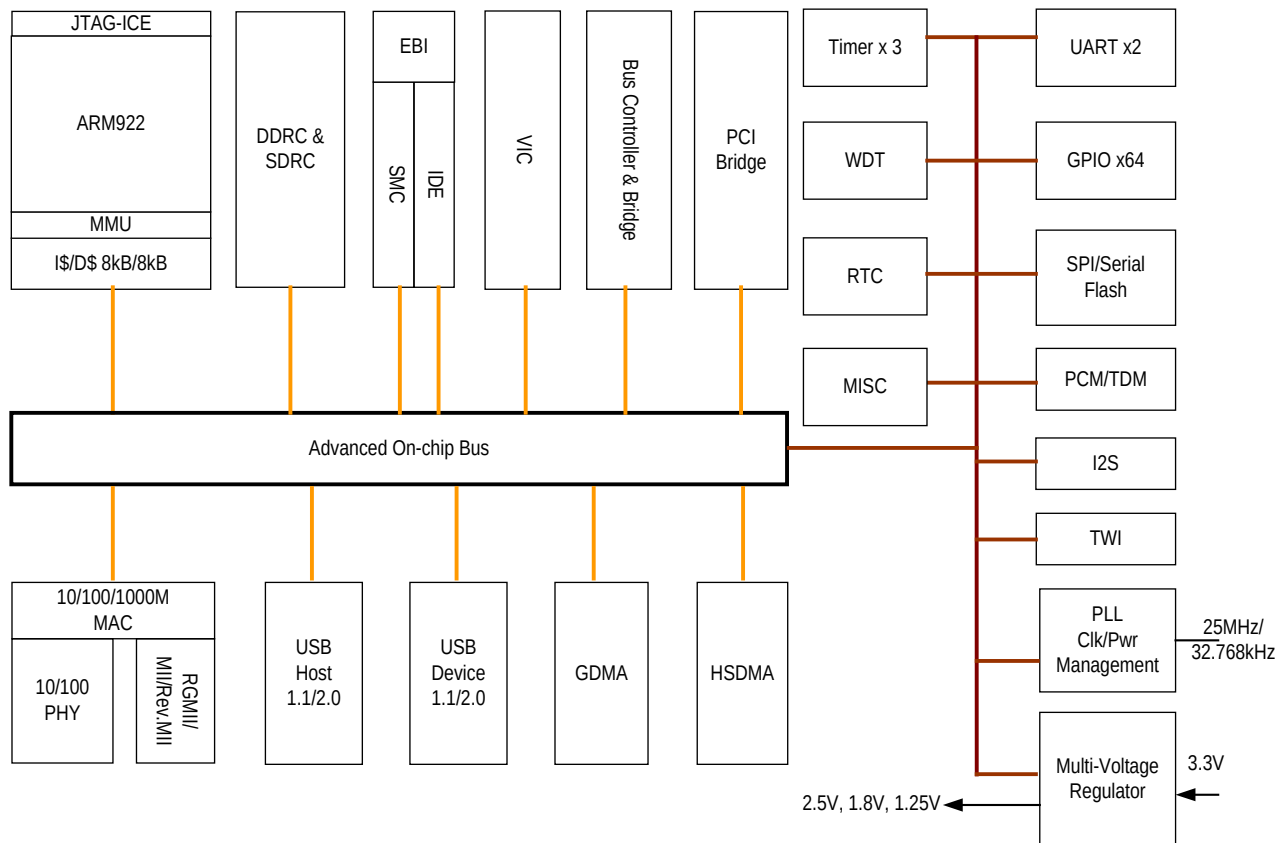
Figure 2. System Block Diagram of Equuleus SoC
