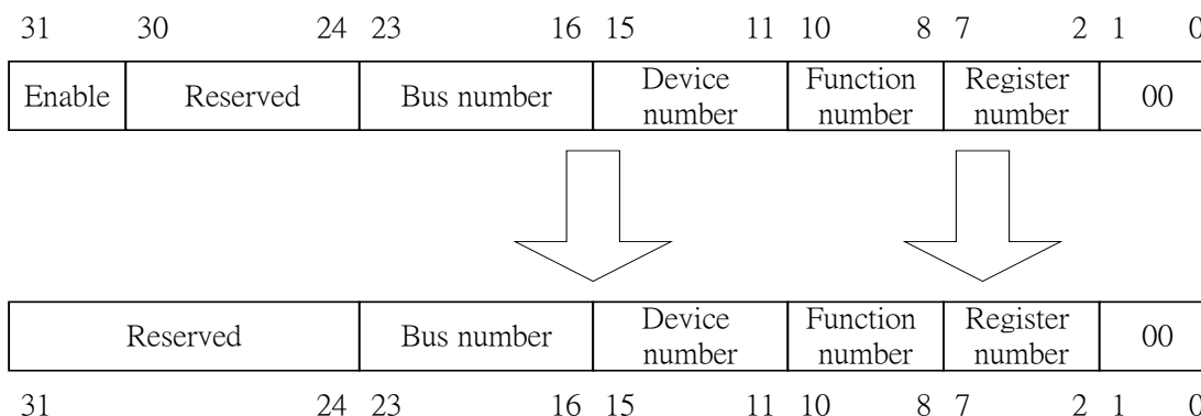
Figure 12. Type 1 Translation
