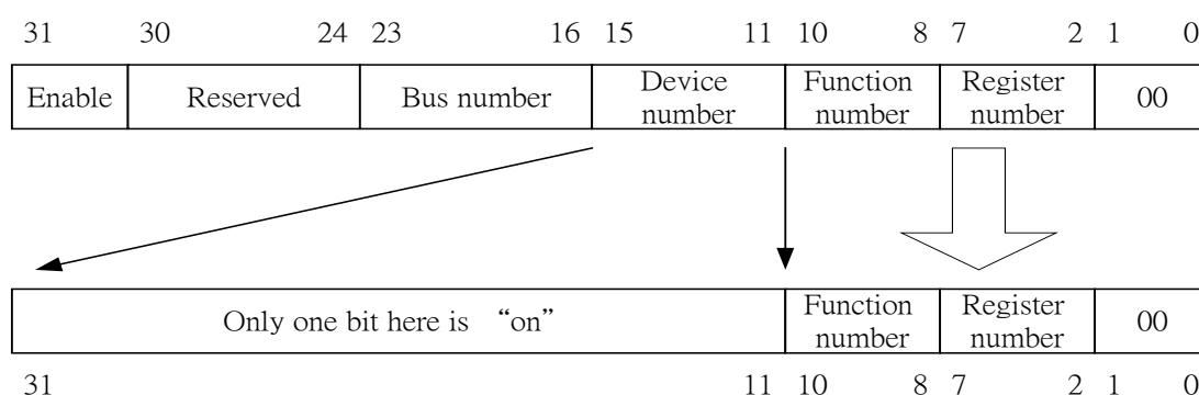
Figure 11. Type 0 Translation
