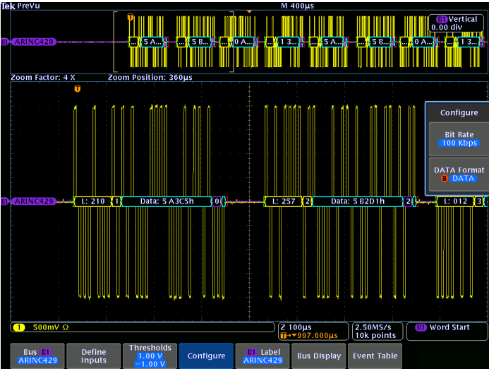
ARINC 429 bus setup, showing configuration entry of bit rate and data format.
