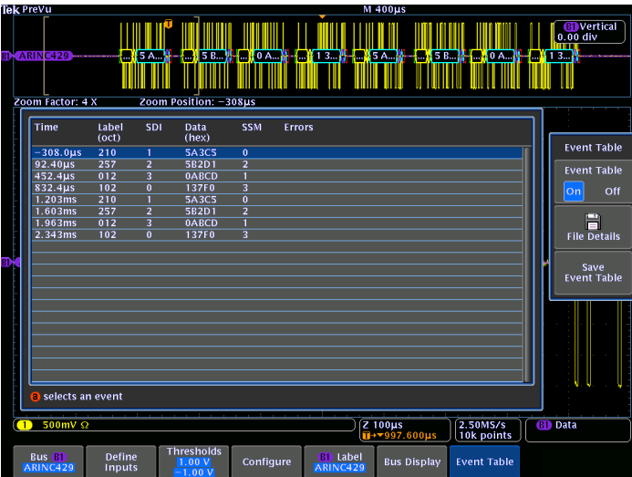
Event table for ARINC 429 bus with all captured packets time stamped and in a tabular view.
