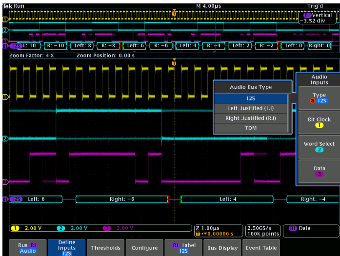
I²S bus setup, showing input configuration options for I²S bus.
