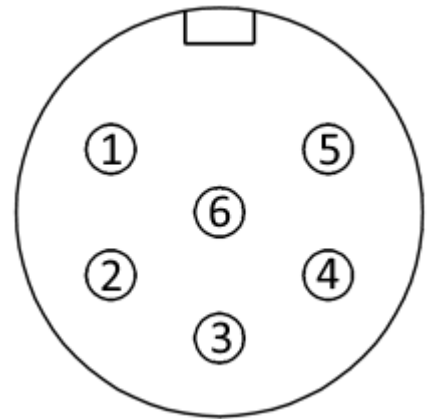
CHOGORI 6-PIN MALE, EXTERNAL VIEW
