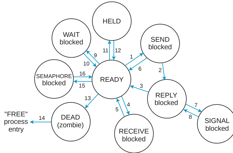
Possible process states in a QNX system.
