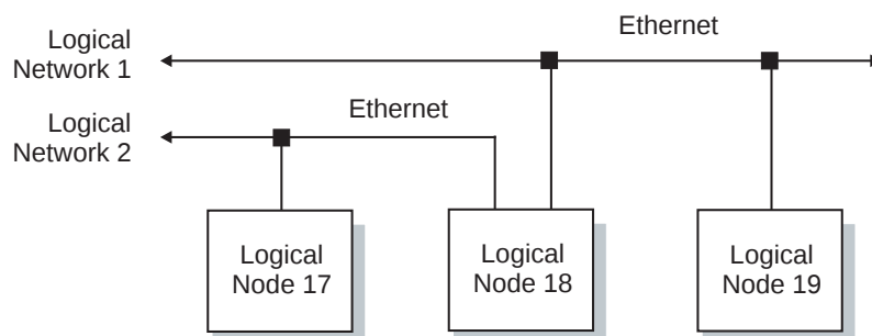
Network bridging between two IEEE 802-based QNX LANs.
