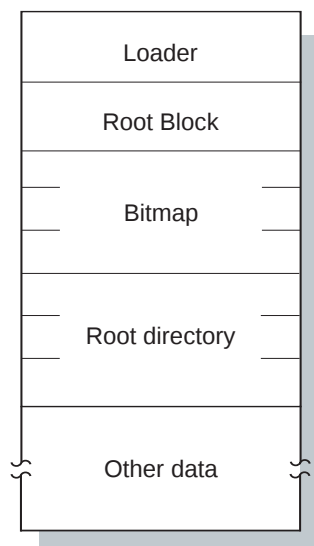
Structure of a QNX filesystem within a disk partition.
