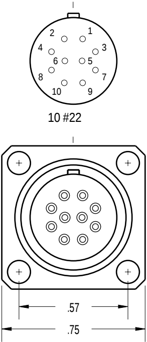
CONTACT CONFIGURATION (BCR FACE VIEW)
