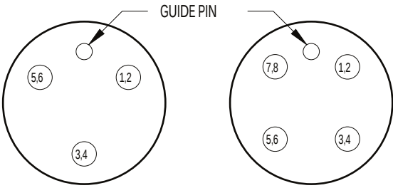
CONTACT CONFIGURATIONS (IEB6/8M FACE VIEWS)
