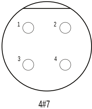
CONTACT CONFIGURATION (BCR FACE VIEWS)
