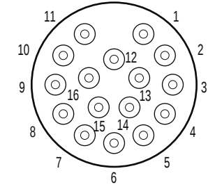
16 CONTACT (MOM NOT AVAILABLE)
