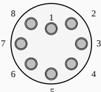
Male Face View Subconn MCIL8M Molded to SO Cable
