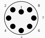
Female Face View Subconn MCBHRASS on custom 1" stem
