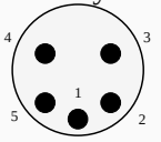
Female Face View Subconn MCIL5F Molded to SO Cable
