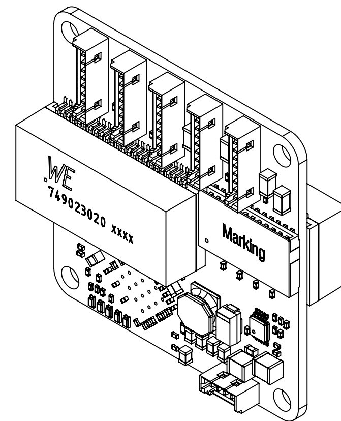
ISOMETRIC VIEW
