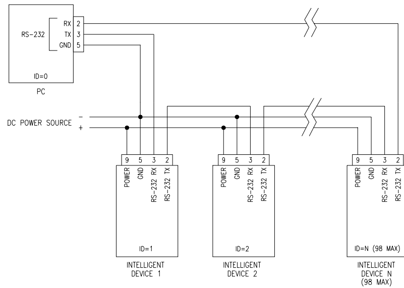
Figure 25. RS-232 serial loop network
