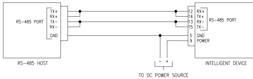
Figure 26. 2-wire RS-485 system, single device
