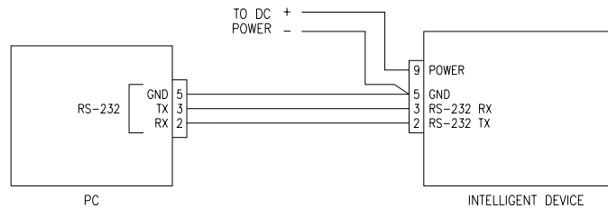
Figure 24. Simple RS-232 wiring diagram
