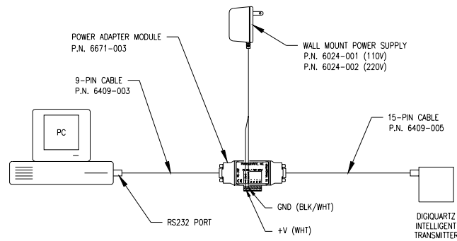
Figure 23. RS-232 wiring diagram using optional RS232/RS485 Power Module Kit
