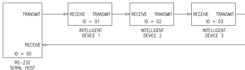
Figure 12. Serial loop network block diagram
