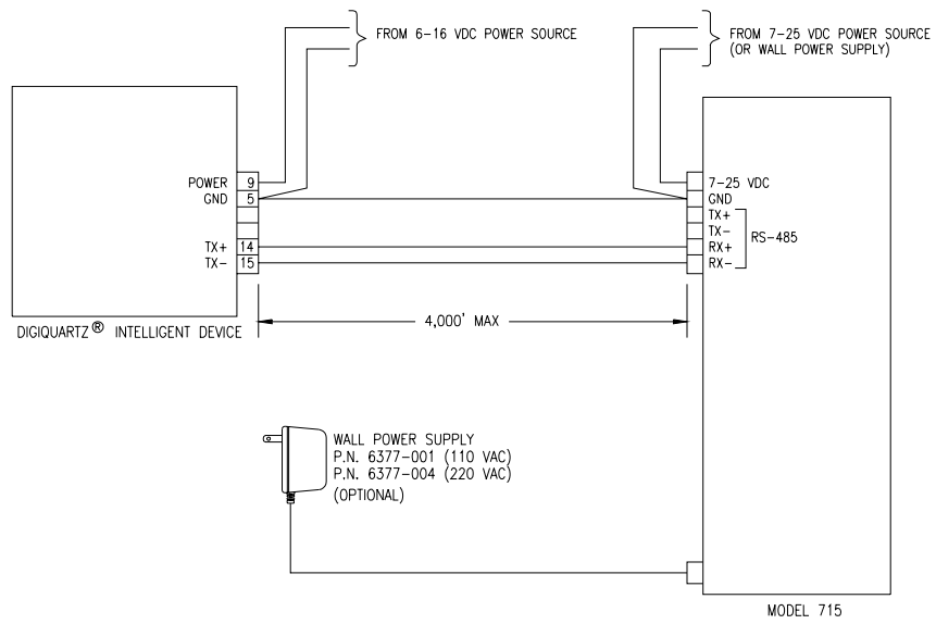
Figure 32. Model 715, RS-485 connection to an Intelligent device
