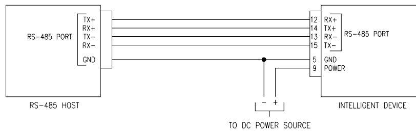
Figure 27. 4-wire RS-485 system, single device
