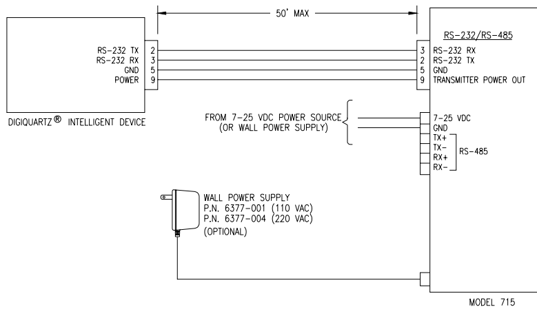
Figure 31. Model 715, RS-232 connection to an Intelligent device
