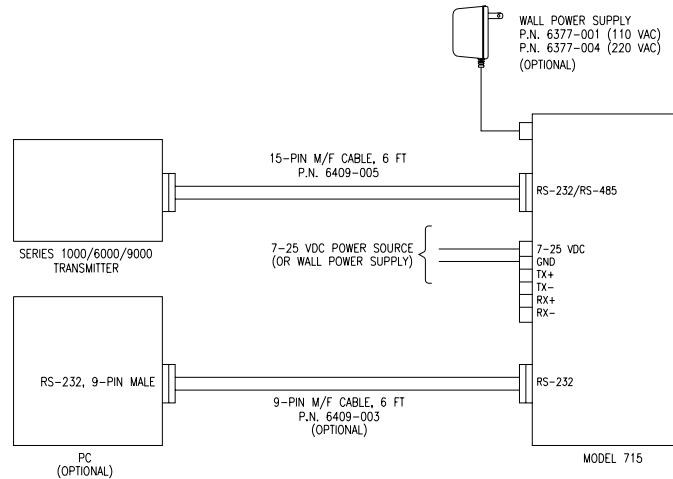
Figure 30. Simple Model 715 / Intelligent transmitter system, w/ optional PC shown
