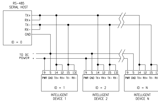
Figure 28. 2-wire RS-485 multi-drop network
