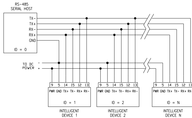
Figure 29. 4-wire RS-485 multi-drop network
