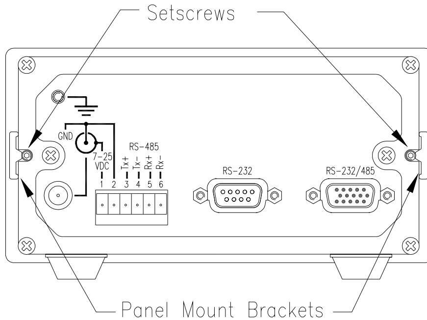
Figure 14. Model 715 rear panel detail
