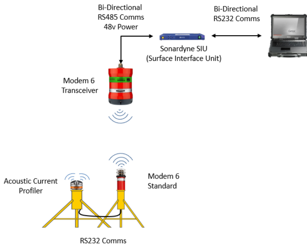
Figure 17 Integration Example 1 System Diagram
