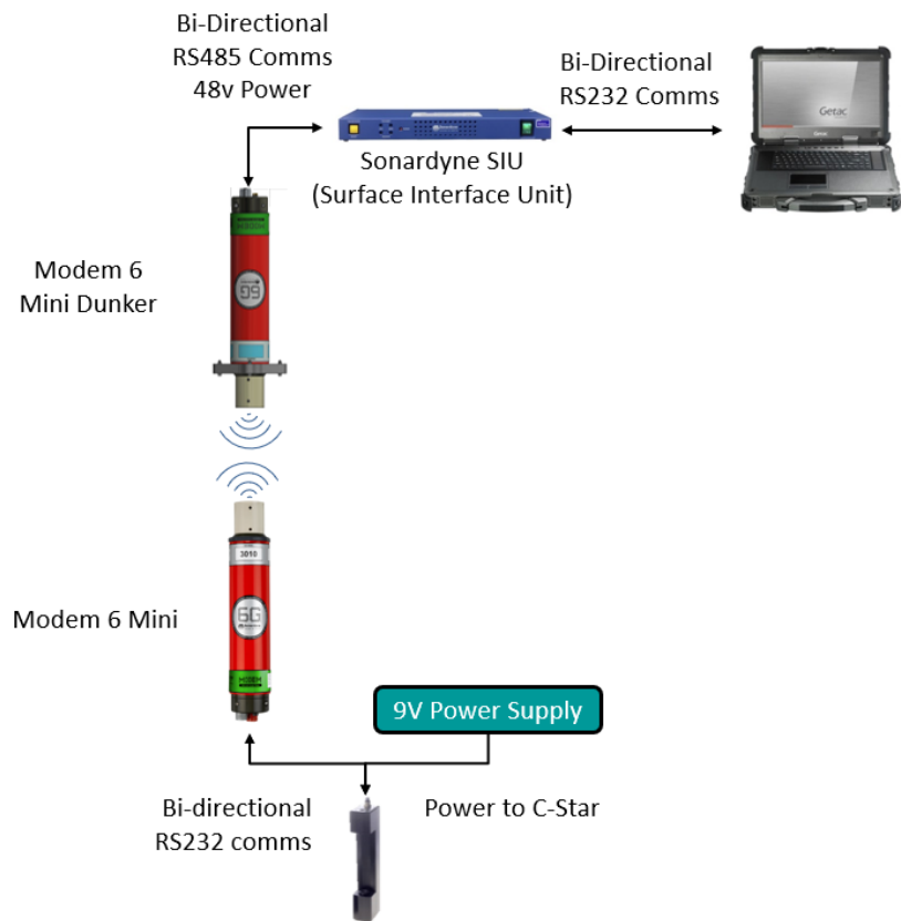
Figure 19 Integration Example 2 System Diagram
