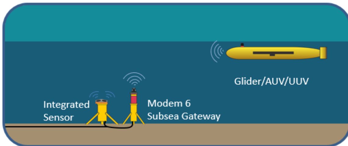
Figure 8 UUV to Subsea Infrastructure Interfacing
