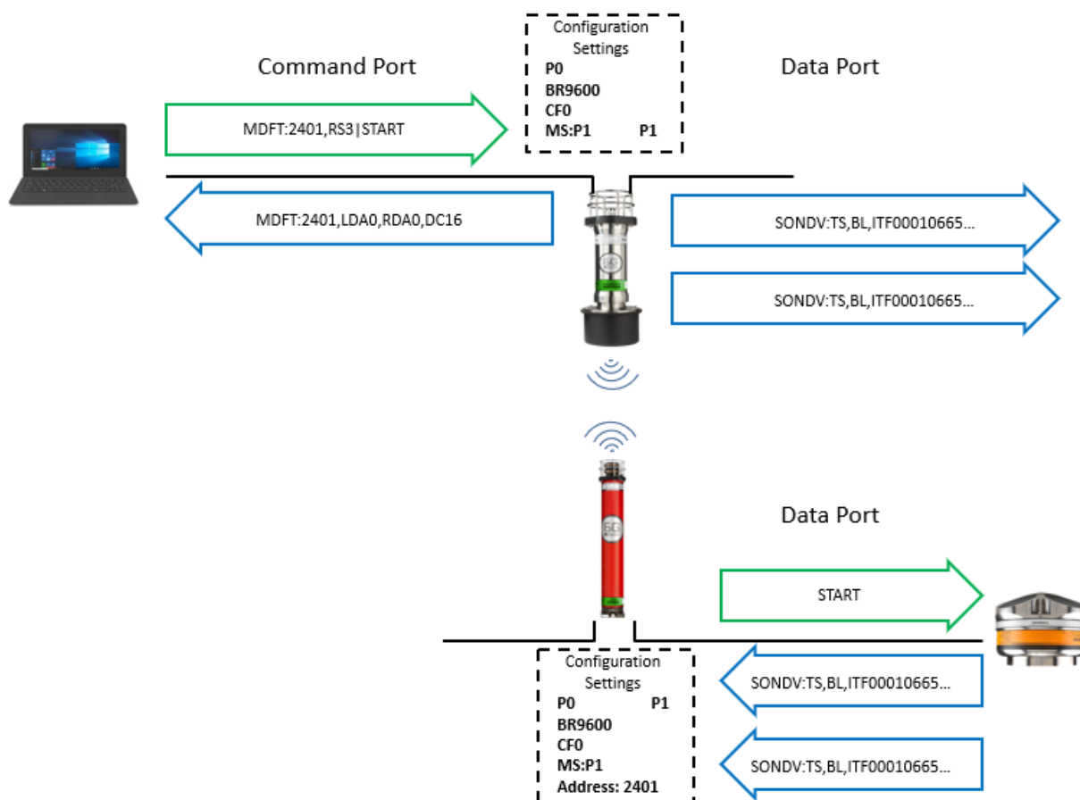
Figure 5 Data Streaming: Fire and Forget System Diagram
