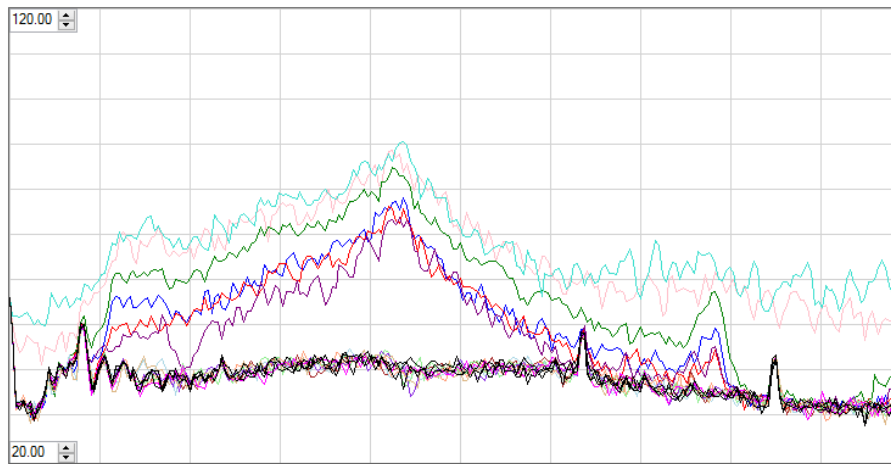
Figure 16 FFT Spontaneous Noise Floor Increases
