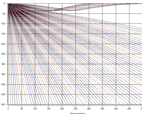
Figure 15 Ray Path Analysis
