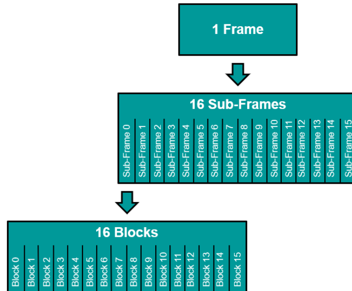
Figure 4 MDFT Frame Data Structure
