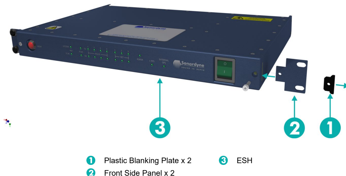
Figure 4-1 Front Rack Mounting Side Panel Installation
