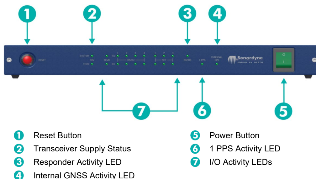
Figure 3-1 Ethernet Serial Hub Front View
