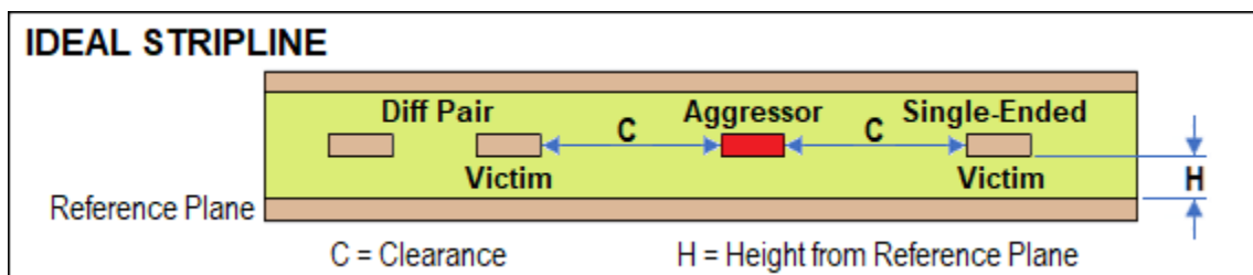
Figure 10.2: Same Layer Coupling – Stripline
