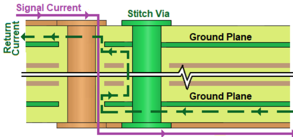
Figure 4.3: Stitch Via Connecting Ground Planes
