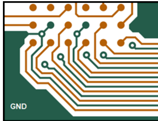
Figure 4.1: Triplets Routing
