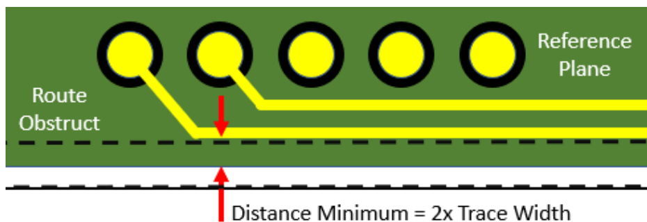
Figure 4.5: Using Route Obstruct
