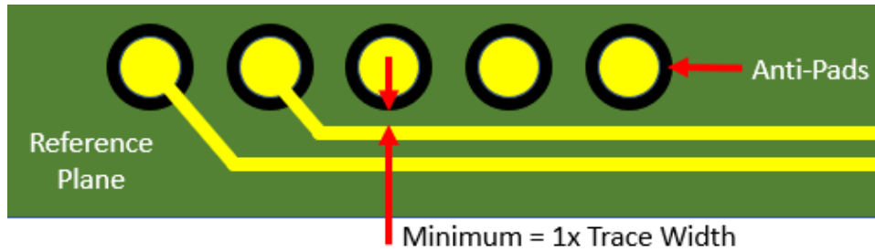
Figure 4.7: Trace to Anti-Pad Constraint
