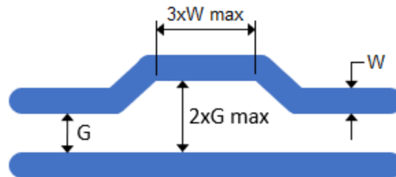
Figure 21.6: Max Spacing of Tuning Bumps
