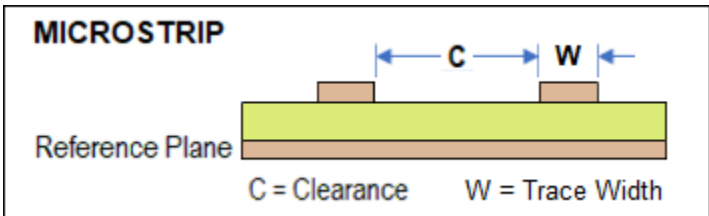
Figure 12.7: Same Net Coupling – Trace Width
