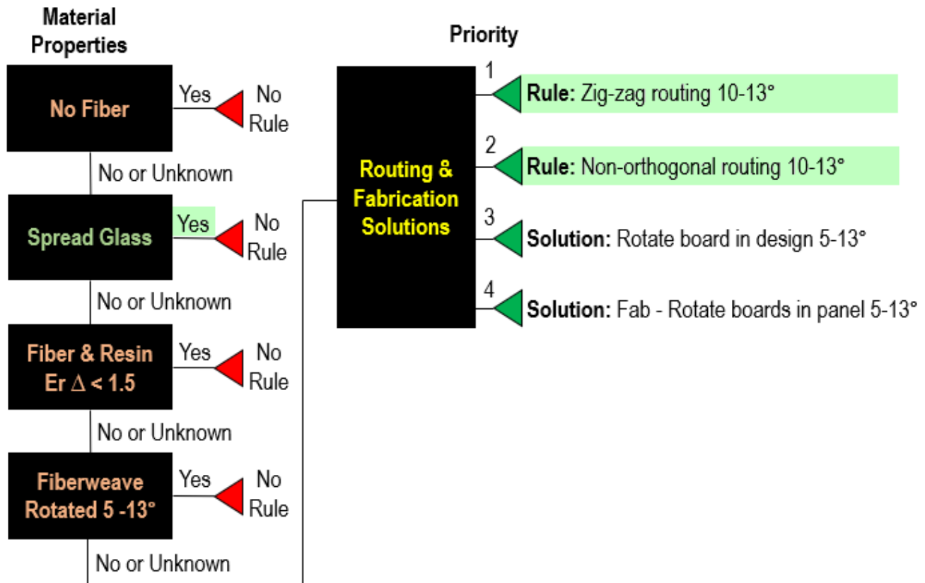
Figure 7.2: Fiberweave Skew
