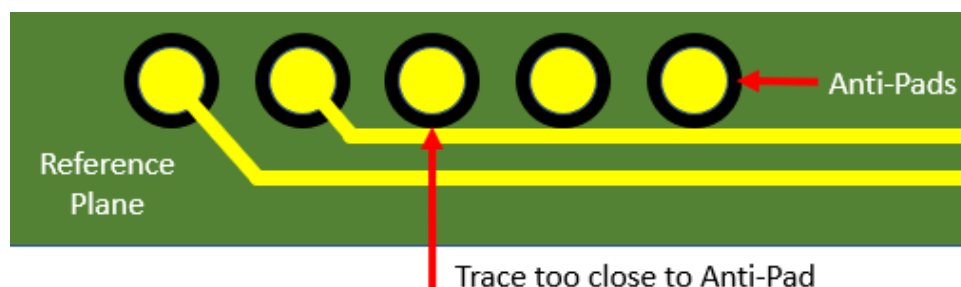
Figure 4.6: Critical Length Trace & Anti-Pads
