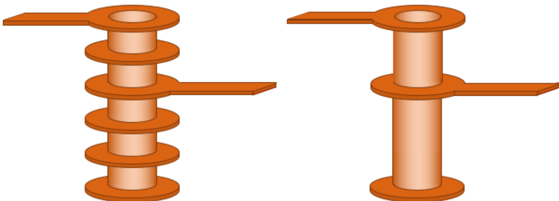
Figure 16.1: Via Before/After Nonfunctional Pads Removed
