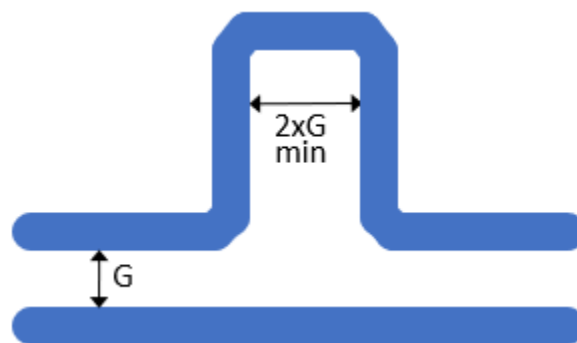
Figure 21.7: Avoid Same-Net Crosstalk
