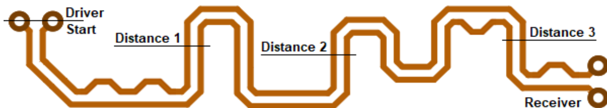
Figure 9.3: Phase Matching Technique
