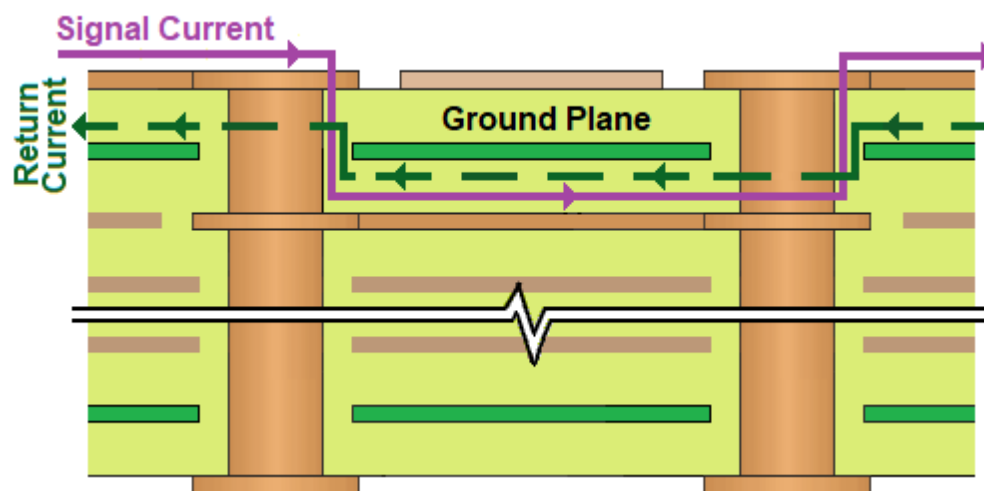
Figure 4.2: Route on Opposite Sides of Reference Plane Layer
