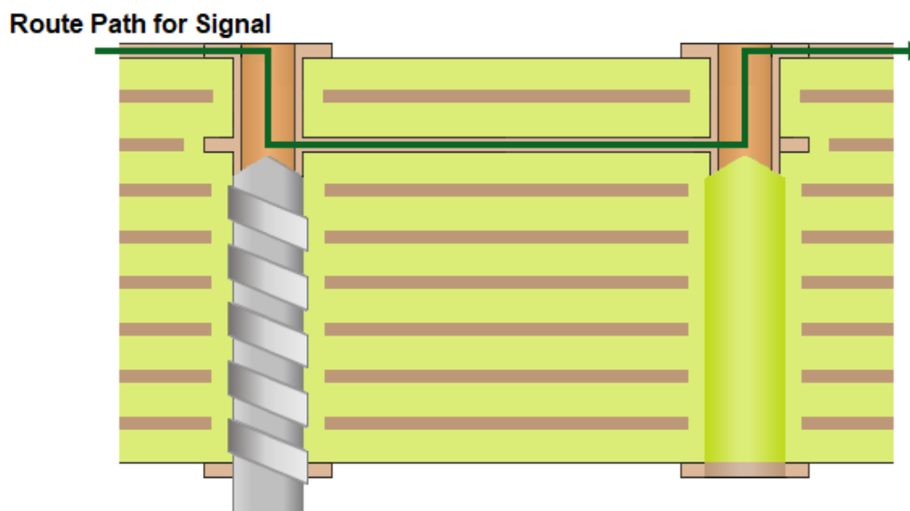
Figure 15.5 Backdrilling
