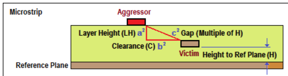
Figure 11.1: Adjacent Layer Coupling – Microstrip
