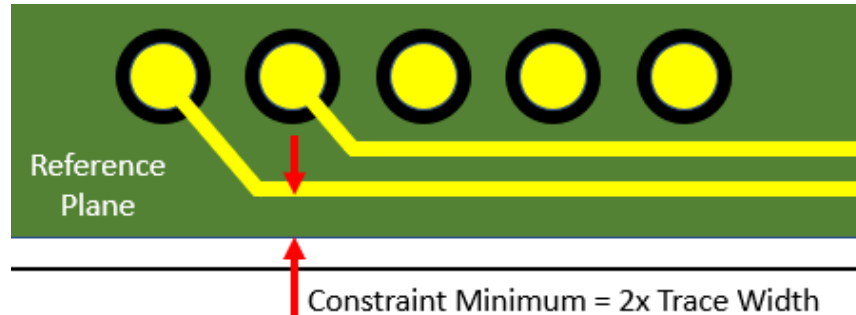
Figure 4.4: Trace to Plane Edge Constraint
