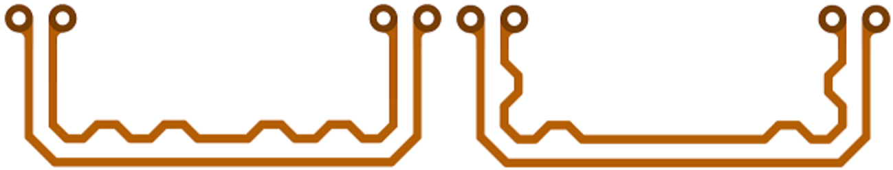
Figure 9.2: Adding Phase Bumps
