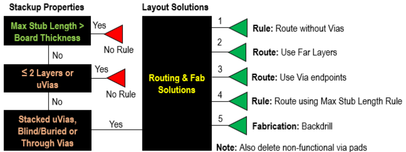
Figure 15.3: Decision Tree for Via Stub Solutions
