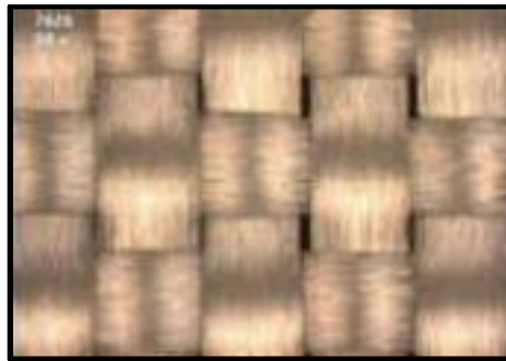
Figure 7.3: 7628 Spread Glass Weave 2
