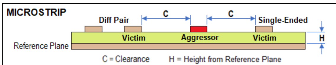
Figure 10.1: Same Layer Coupling – Microstrip
