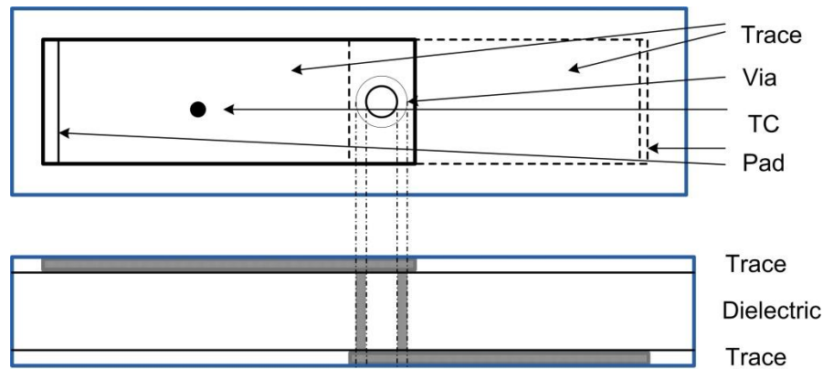
Figure 1 Thermal model of trace with via. (Not to scale)
