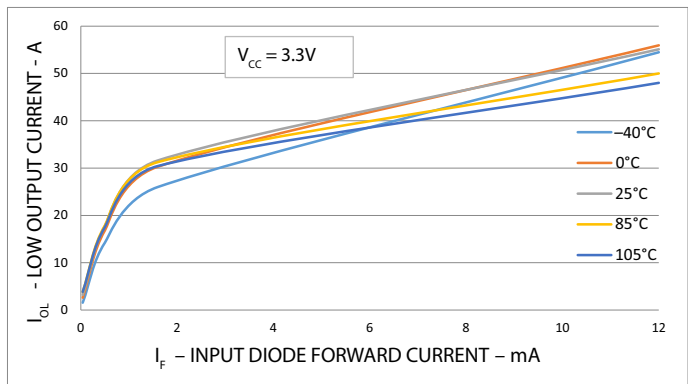
Figure 7: Logic Low Output Current vs. Temperature
