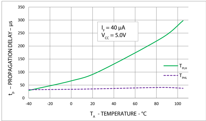
Figure 8: Typical Propagation Delay vs. Temperature
