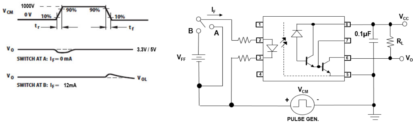
Figure 15: Test Circuit for Transient Immunity and Typical Waveforms
