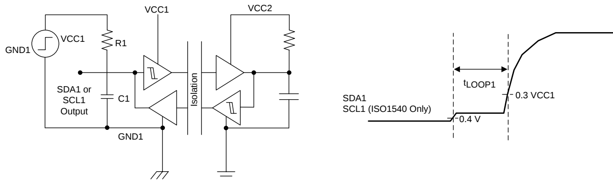
Figure 20. t_{\text{Loop1}} Setup and Timing Diagram
