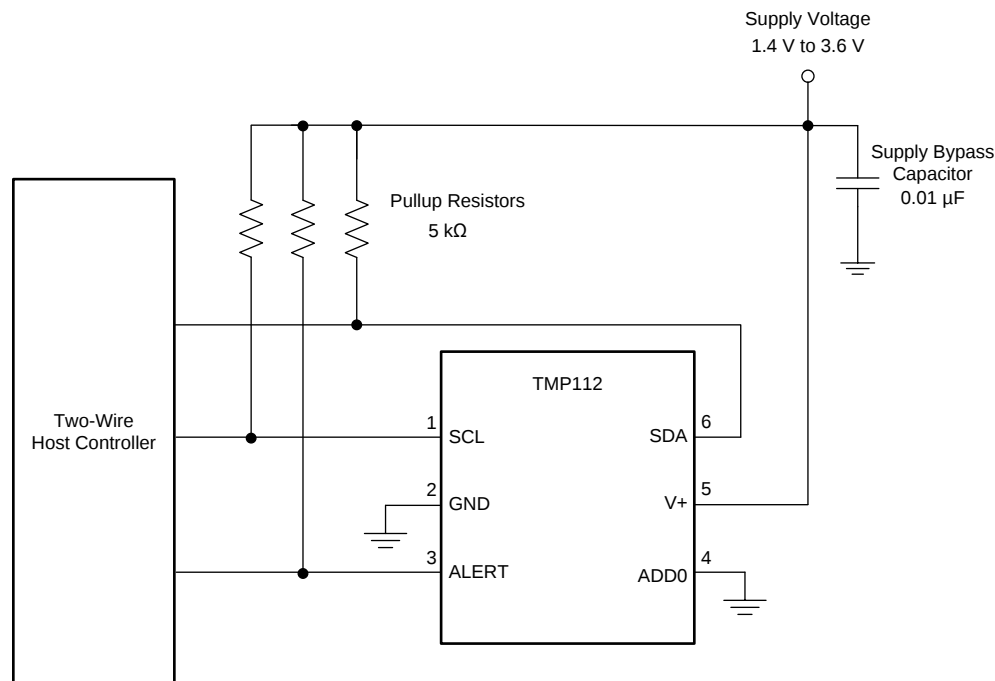
Figure 17. Typical Connections
