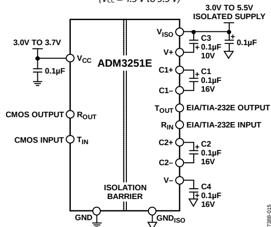
Figure 15. Typical Operating Circuit with the DC-to-DC Converter Disabled ( V_{CC} = 3.0 V to 3.7 V)
