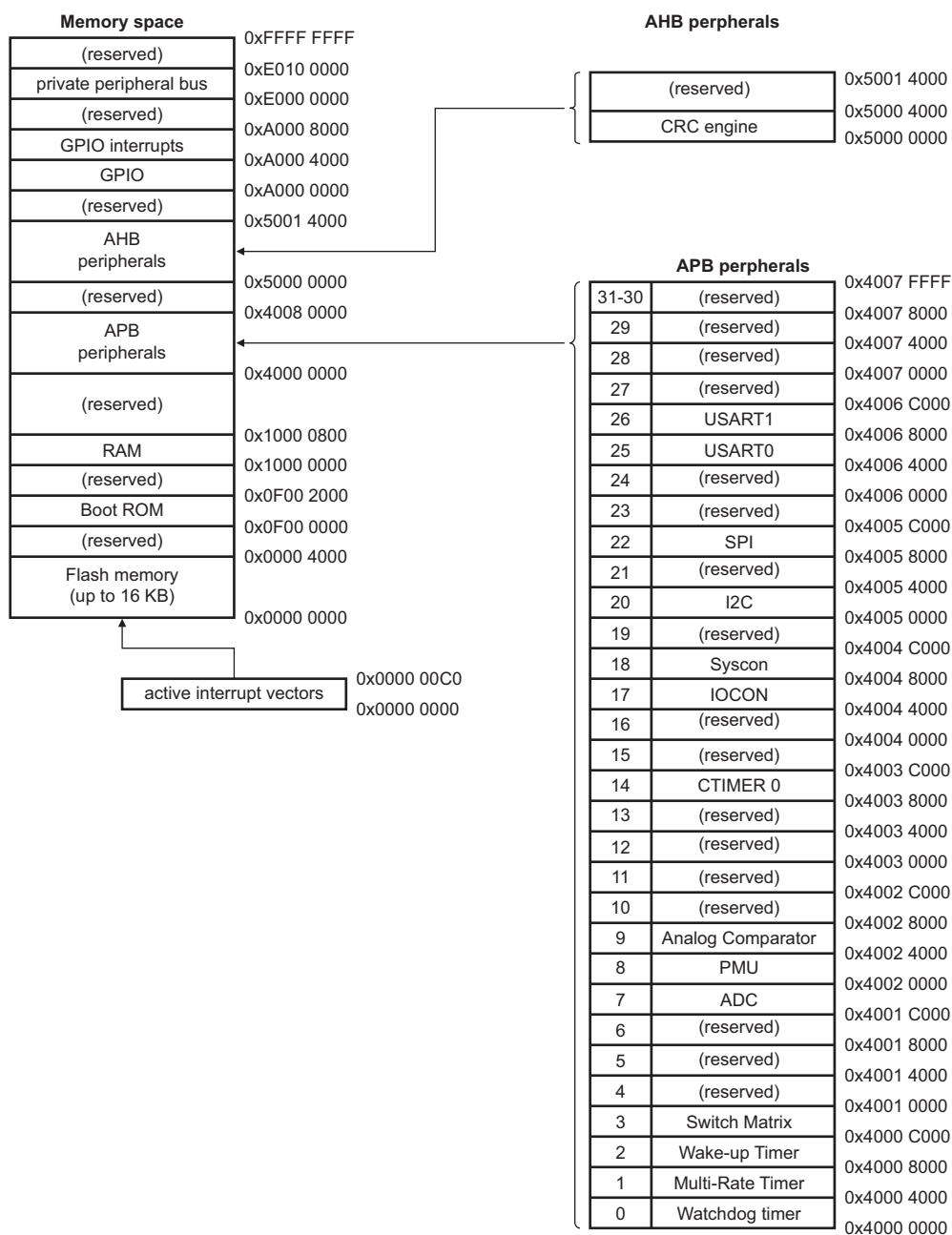
Fig 9. LPC802 Memory mapping
