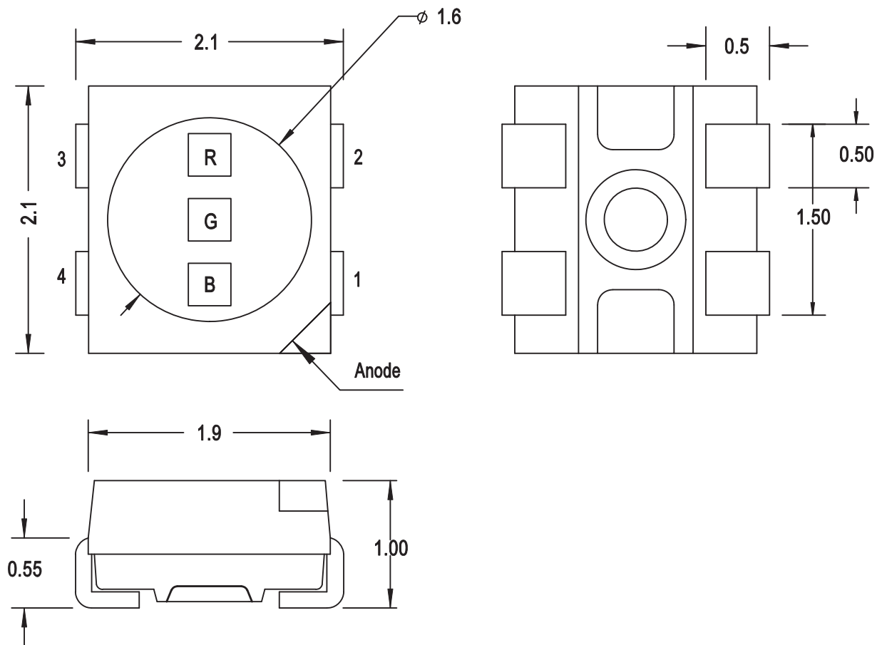
Figure 1: Package Drawing
