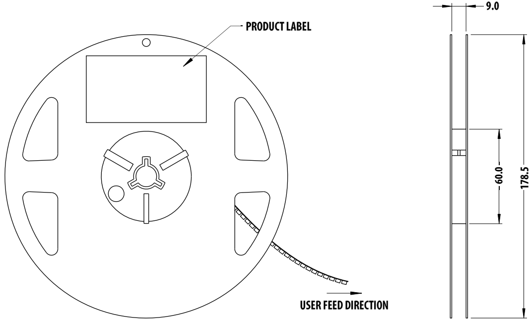
Figure 14: Reel Dimensions
