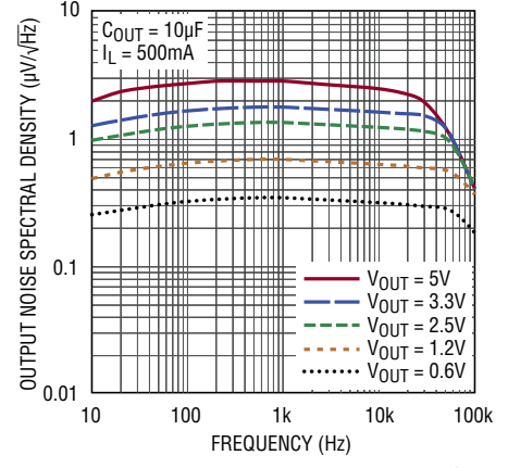
Output Noise Spectral Density C_{REF/BYP} = 0 , C_{FF} = 0
