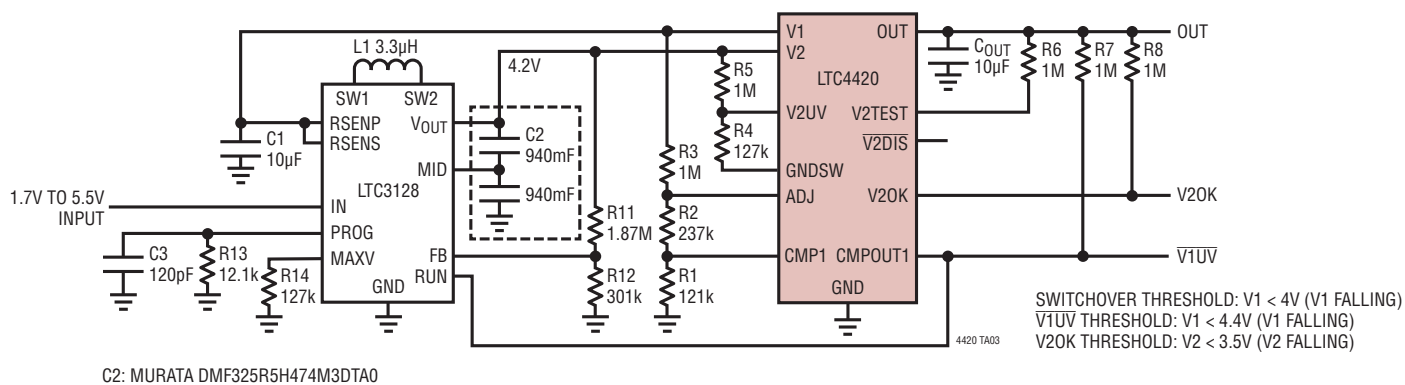
SuperCap Backup with SuperCap Charging
