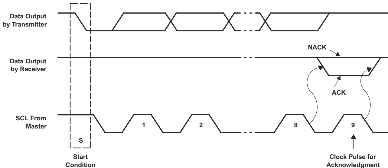
Figure 8-3. Acknowledgment on I 2 C Bus
