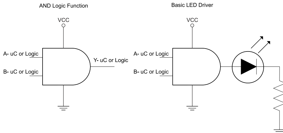
Figure 10-1. Typical Application
