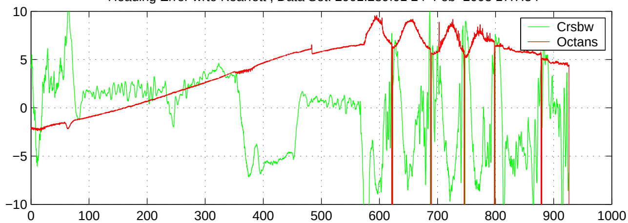
Heading Error wrto Kearfott ; Data Set: 2001.289.01 24-Feb-2003 17:7:34
