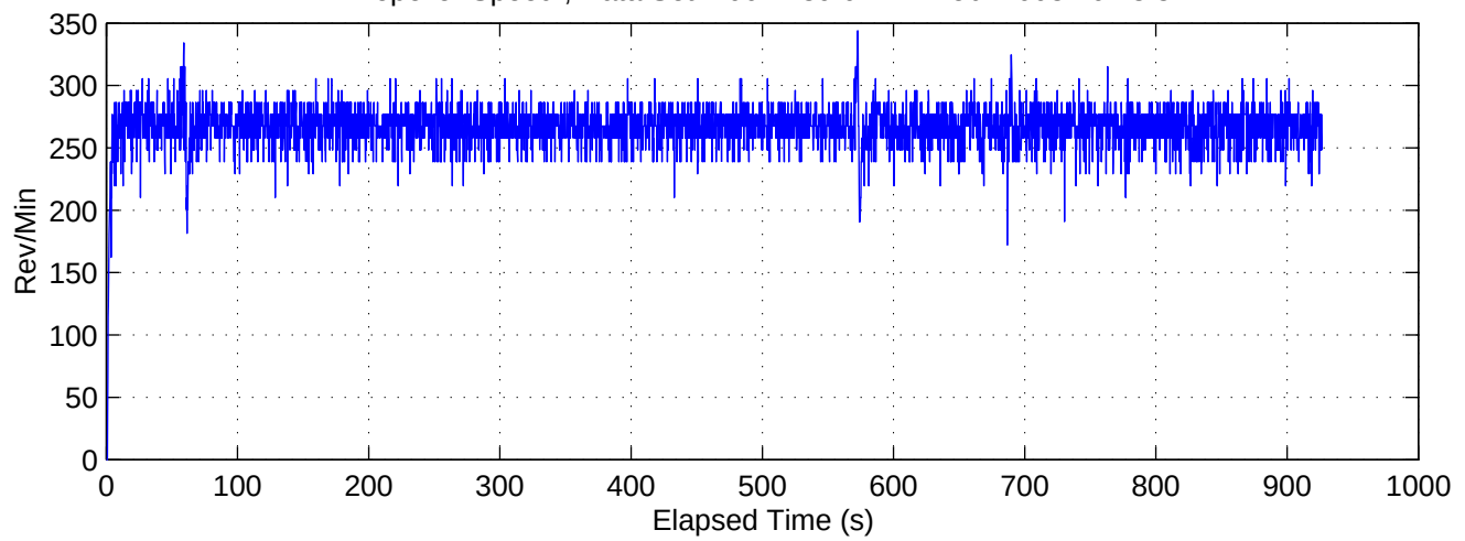
Propeller Speed ; Data Set: 2001.289.01 24-Feb-2003 16:48:31
