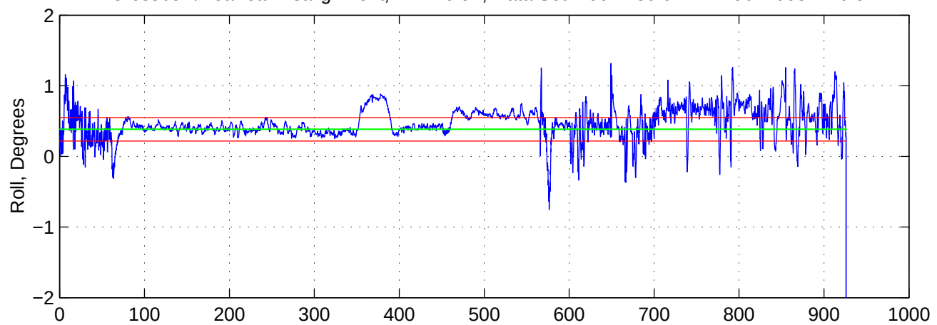
Crossbow/Kearfott Misalignment; 2-1 Euler ; Data Set: 2001.289.01 24-Feb-2003 17:6:3
