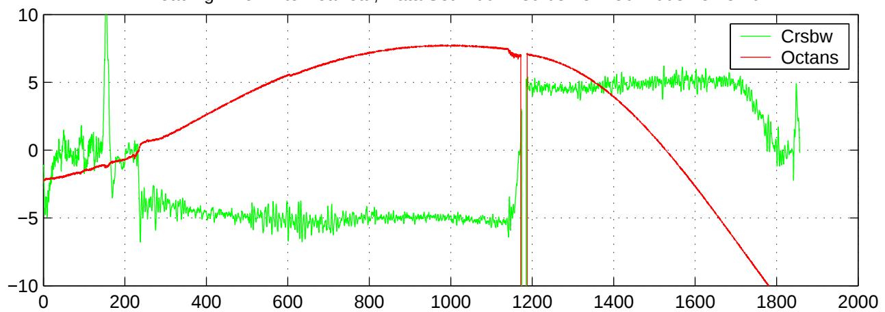
Heading Error wrto Kearfott ; Data Set: 2001.289.03 25-Feb-2003 15:18:10
