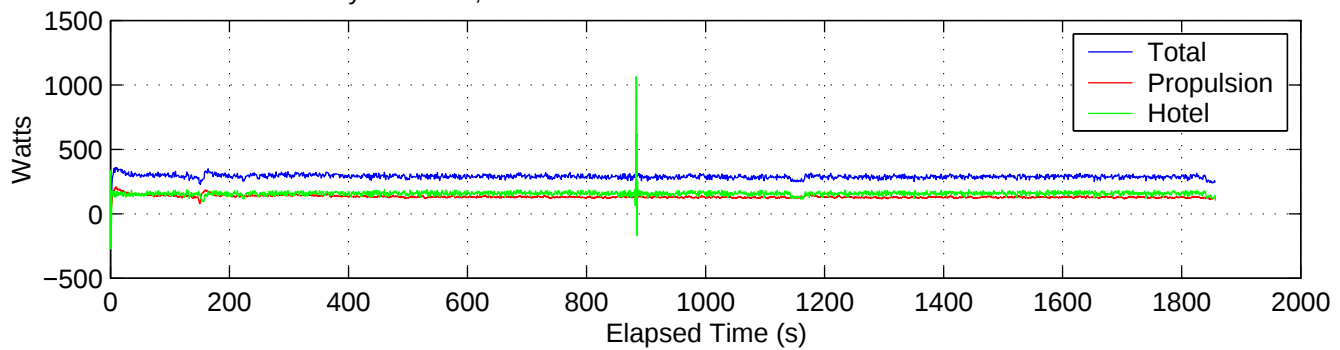
Metrabyte Power ; Data Set: 2001.289.03 Plotted on 25-Feb-2003 15:12:5
