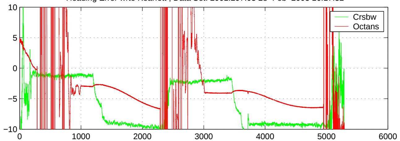
Heading Error wrto Kearfott ; Data Set: 2001.297.03 28-Feb-2003 16:17:32
