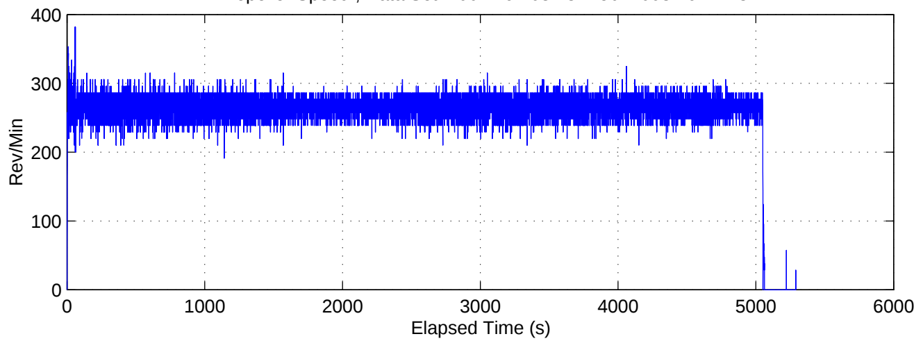
Propeller Speed ; Data Set: 2001.297.03 28-Feb-2003 16:17:48
