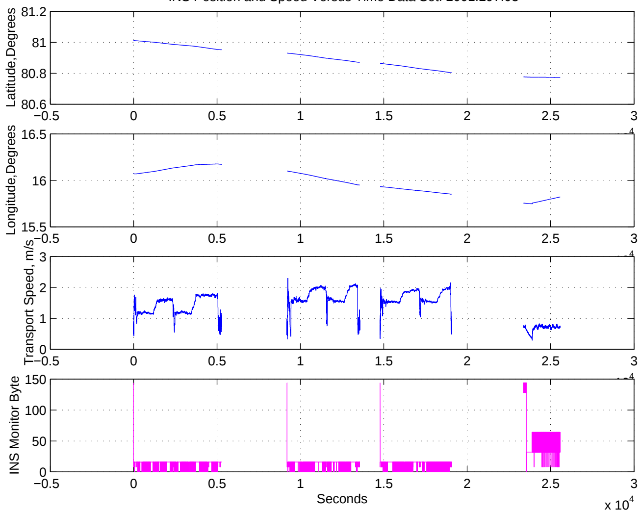
INS Position and Speed Versus Time Data Set: 2001.297.03
