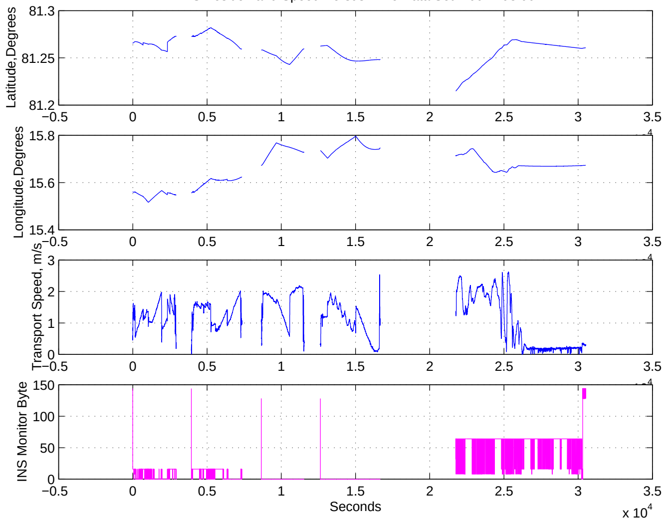
INS Position and Speed Versus Time Data Set: 2001.298.00
