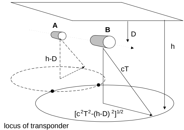
Fig. 1. A and B represent two poses of an AUV flying at depth D over flat terrain in a water column of depth h with sound velocity c . A single TOF constrains the a transponder to lie on a circle centered on the vehicle. In general two such TOF's constrain the transponder to lie at one of two circle intersections producing a “baseline” ambiguity.
