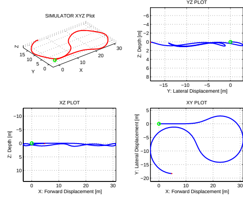
Fig. 6: REMUS Simulator Data: Vehicle trajectory for vehicle response in the horizontal plane
