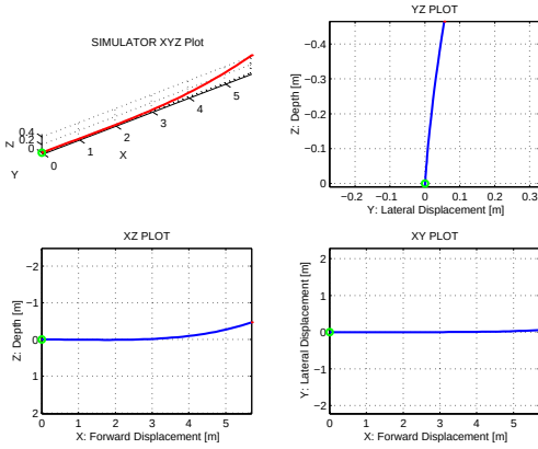
Fig. 8: REMUS Simulator Data: Vehicle trajectory for vehicle pitching up
