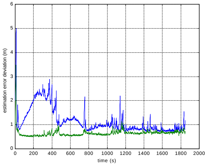
Fig. 6 – Length of the axes of the estimation error ellipse.
